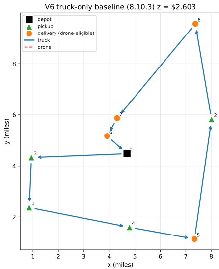
(a) Truck-only PDP, z = \$2.60 .
